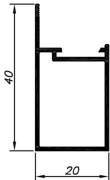
MP-300 1.782 Kg/Barra 6m
