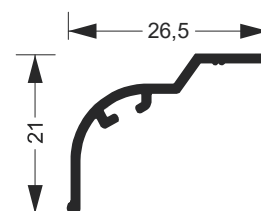
GNS-041 0.838Kg/Barra 6m
