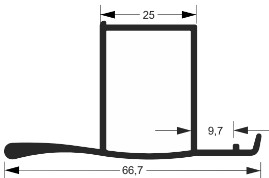
SUP-2650 4.158Kg/Barra 6m
