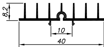
LM-100 1.290 Kg/Barra 6m
