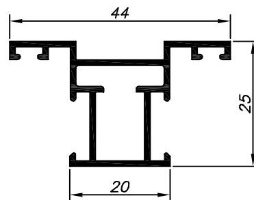
25-308 2.720 Kg/Barra 6m
