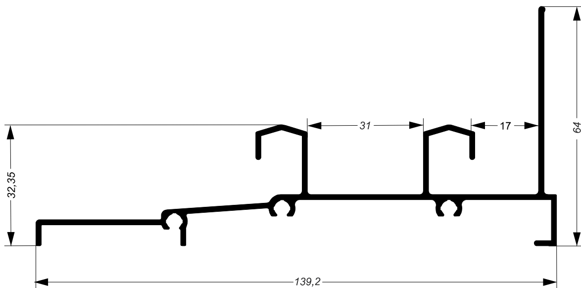
NOE-035 8.019Kg/Barra 6m
