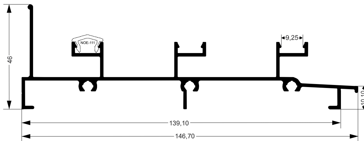
NOE-116 9,223Kg/Barra 6m
