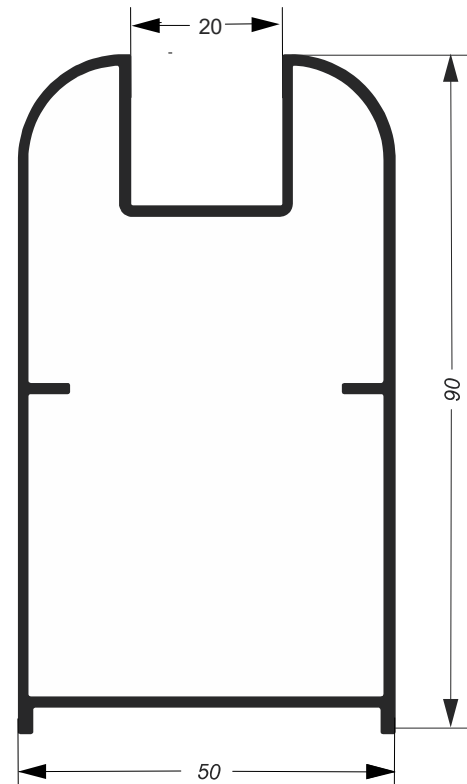
POR-292 8,454kg/6m
