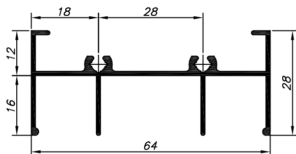
MP-357 3.430 Kg/Barra 6m
