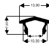
NOE-111 0,580Kg/Barra 6m
