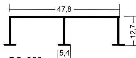
DS-033 1,200 kg/Barra 6m
