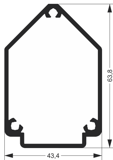
GNS-049 6.435Kg/Barra 6m
