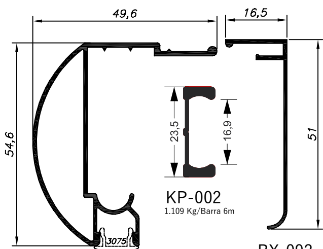
BX-091T 3,720 Kg/Barra 6m
