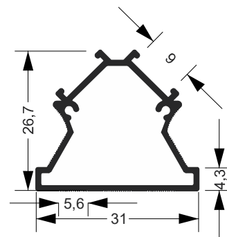
LM-003 1.620 Kg/Barra 6m
