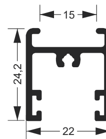
SUP2572 2.158Kg/Barra 6m
