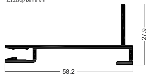
NOE-203 2,874Kg/Barra 6m
