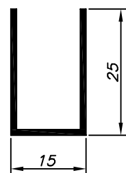
PU-040 1,190 Kg/Barra 6m
