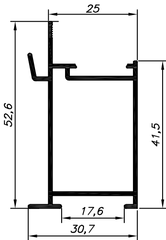
SU-282 2,675 Kg/Barra 4,6m
