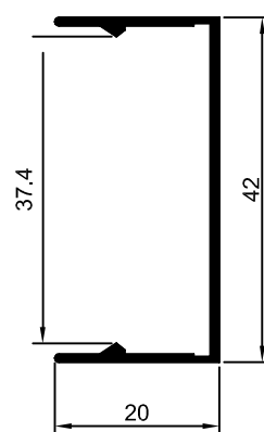
FC-013 1.420 Kg/BARRA 6m
