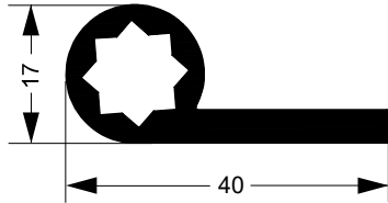
11.0085 4.006 Kg/Barra 6m
