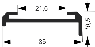
DES-112 1,558Kg/Barra 6m
