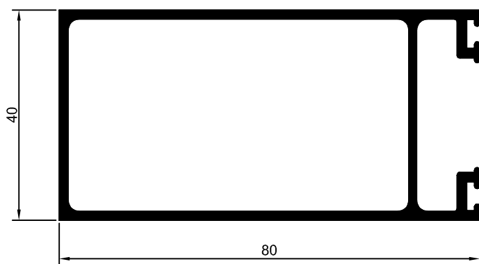
FC-012 6.700 Kg/BARRA 6m Borracha GUA008
