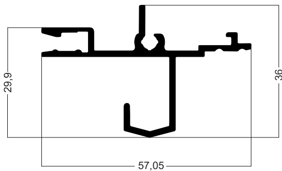
NOE-218 3,745Kg/Barra 6m
