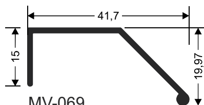
MV-069 1,404 kg/Barra 6m
