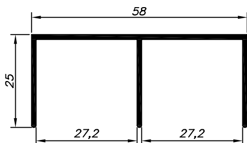
MV-036 2.950 Kg/Barra 6m
