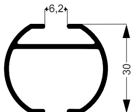
TRI-044 1,842Kg/Barra 6m
