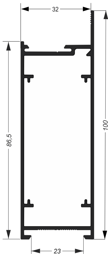
NOE-042 6,380Kg/Barra 6m
