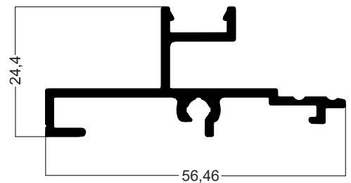
NOE-216 3,343Kg/Barra 6m
