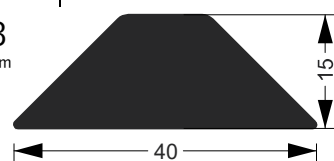
01-0183 7.075Kg/Barra 6m
