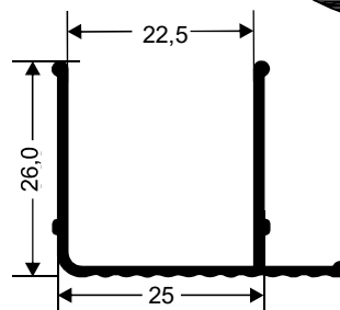
GNS-013 1.788 Kg/Barra 6m
