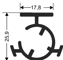
MCG-001 2.930 Kg/Barra 6m
