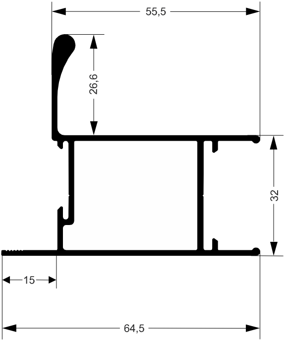
NOE-017 5,683Kg/Barra 6m
