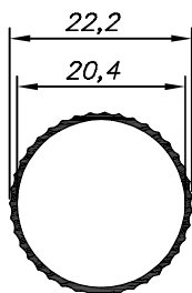
PTF-0022 0.840 Kg/Barra 6m
