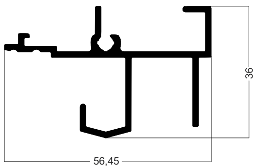
NOE-219 4,264Kg/Barra 6m
