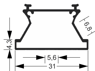
LM-004 1.426 Kg/Barra 6m
