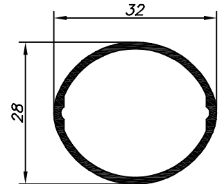
ALU-005 1.734 Kg/Barra 6m
