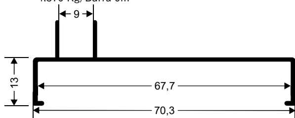
GNS-004 2.448 Kg/Barra 6m
