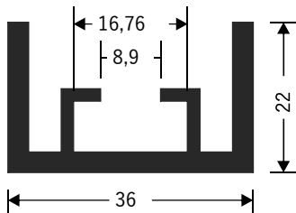
LM-104 4.560 kg/Barra 6m
