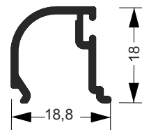
NOE-026 1.069Kg/Barra 6m
