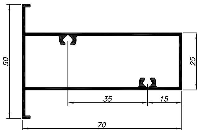
FC-070 5.010 Kg/Barra 6m
